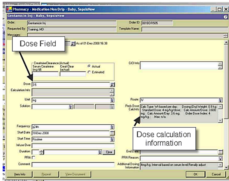
Fig. 5 Artulatory distance: screen layout
