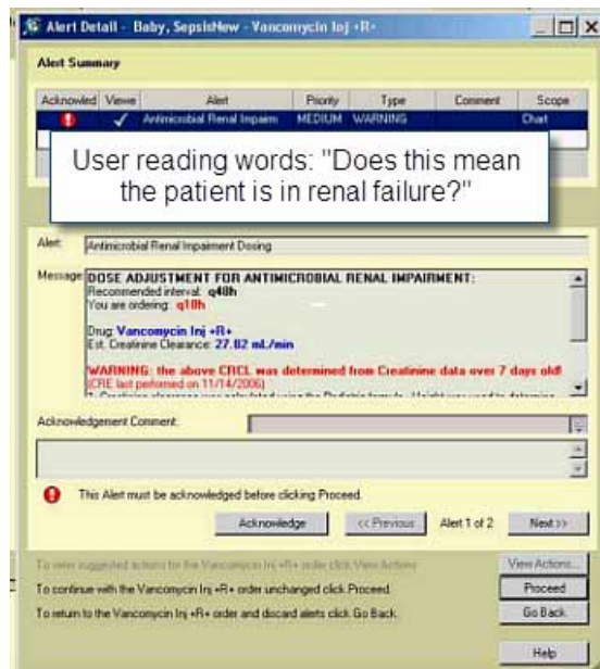
Fig. 6 Screen shot illustrating semantic distance
