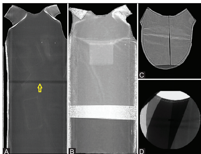
Figure 3 (A-D): Computed tomography (CT) and fluoroscopic images showing defects in protective apparels. (A) Arrow showing a dark line indicating fragility. (B) Nonuniformity of material. (C) Manufacturing defect in thyroid collar. (D) Different combination of lead equivalent material
