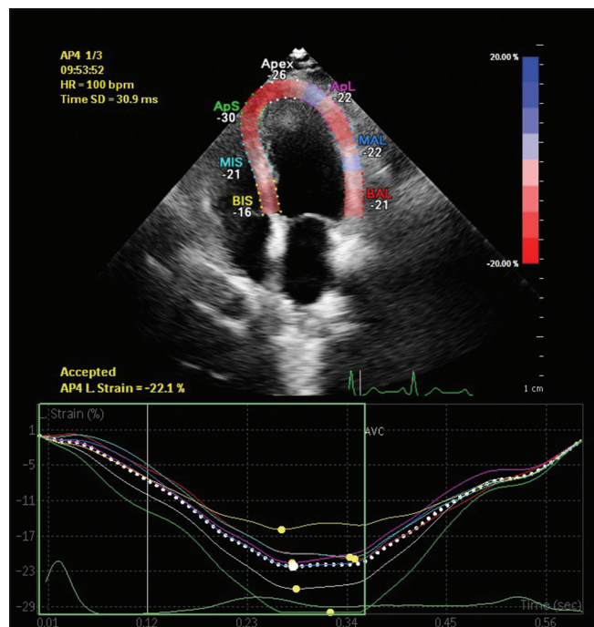
Figure 1: Speckle tracking echocardiography illustrating global longitudinal strain from the apical long-axis four-chamber-view, showing normal left ventricular segmental strain pattern. The color of each trace corresponds to anatomical points on the two-dimensional color image above. The white-dotted line represents average strain
