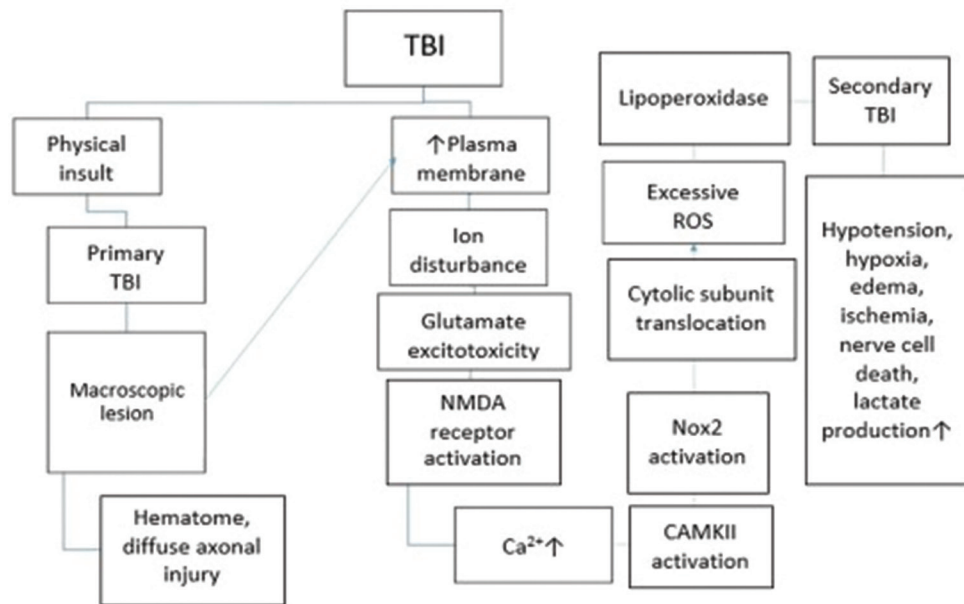
Figure 1: Pathophysiology of traumatic brain injury. TBI: Traumatic brain injury, NMDA: N-methyl-D-aspartate, \text{Ca}^{2+} : Calcium, CaMKII: Calmodulin-dependent protein kinase type II, Nox2: NADPH oxidase, ROS: Reactive oxygen species
