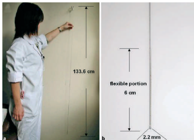
Figure 1 The “styler” is made of stainless steel and is 133.6 cm in length (a). It is 2.2 mm in diameter, and at the tip there is a 6-cm flexible section, which protects the forceps channel (b).
