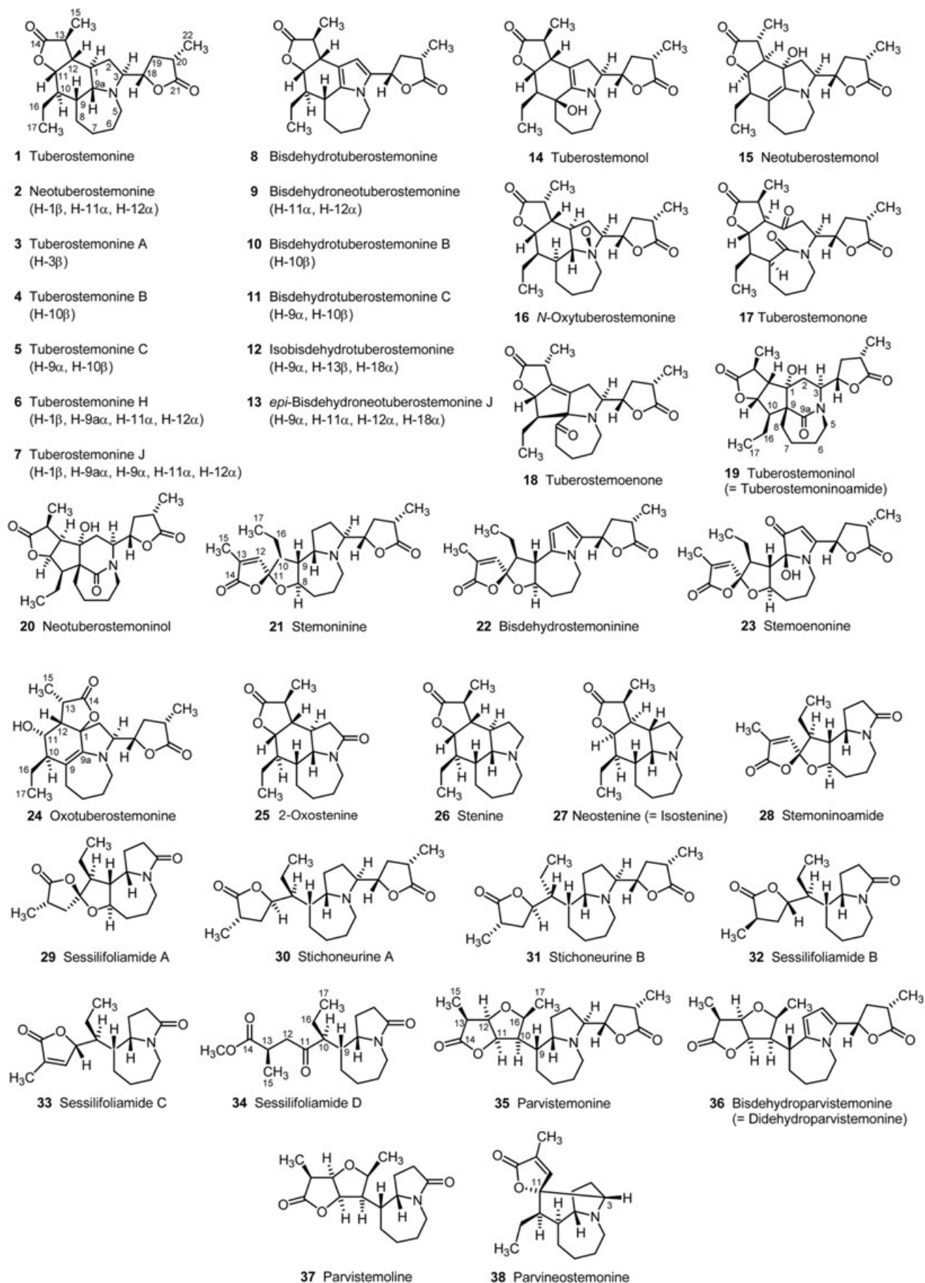
Fig. 2 Stichoneurine-type alkaloids.
