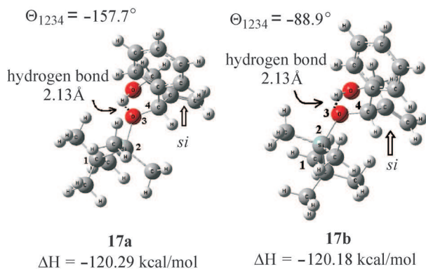
Figure 2 Minimized conformations for the silylated allylic diol 17
