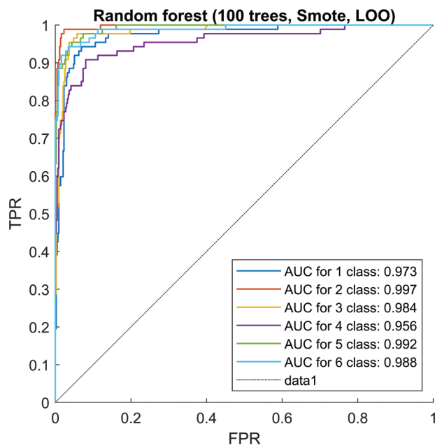
Fig. 2 After generating artificial cases for balancing the class distribution, ROC curves and AUC values for the classification of six classes. AUC, area under the curve; ROC, receiver operating characteristic.
