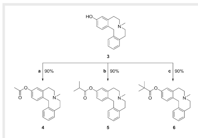
► Fig. 2 Synthesis of 3 ester derivatives/ Reagents and conditions: a NaH, acetyl chloride, 0 °C→rt, CH 2 Cl 2 , 30 min; b NaH, isobutyryl chloride, 0 °C→rt, CH 2 Cl 2 , 30 min; c NaH, pivaloyl chloride, 0 °C→rt, CH 2 Cl 2 , 30 min
