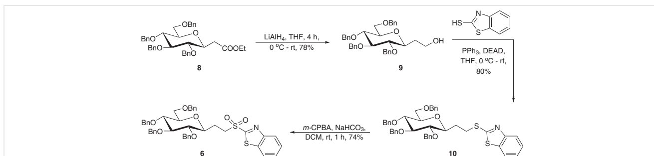
Scheme 1 Synthesis of sulfone building block 6
