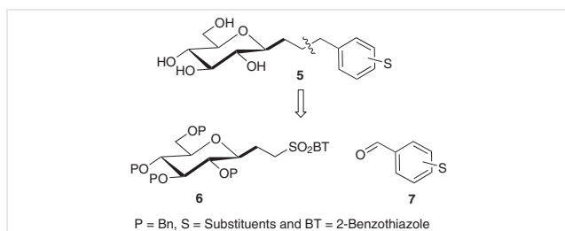
Figure 2 Retrosynthetic analysis of targeted C-glucoside analogues 5
