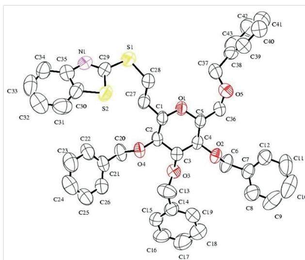
Figure 3 ORTEP diagram of sulfide 10
