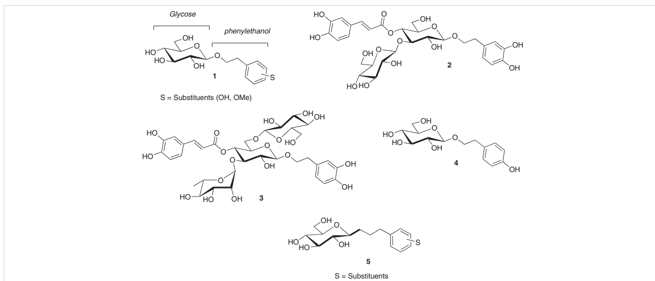
Figure 1 Naturally occurring PEGs and targeted synthetic analogues 5
