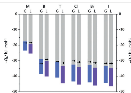
Figure 4 Comparison of the binding or negative dissociation energy -D_0 released when the alcohols M, B, T, Cl, Br, and I attach to the hydroxy esters G and L (full bars), and one quarter of it (colored bar sections), with transmissive (→) and blocking (←) barrier heights for insertion. All values are computed at the B3LYP-D3(BJ)/def2-TZVP level and include a harmonic zero-point correction. For M, the barriers are so low that transmission is granted (see SI, Figure S4). For the heavier systems, it is observed that transmission to a downhill insertion complex is dominant when the barrier does not exceed about one quarter of D_0 .
