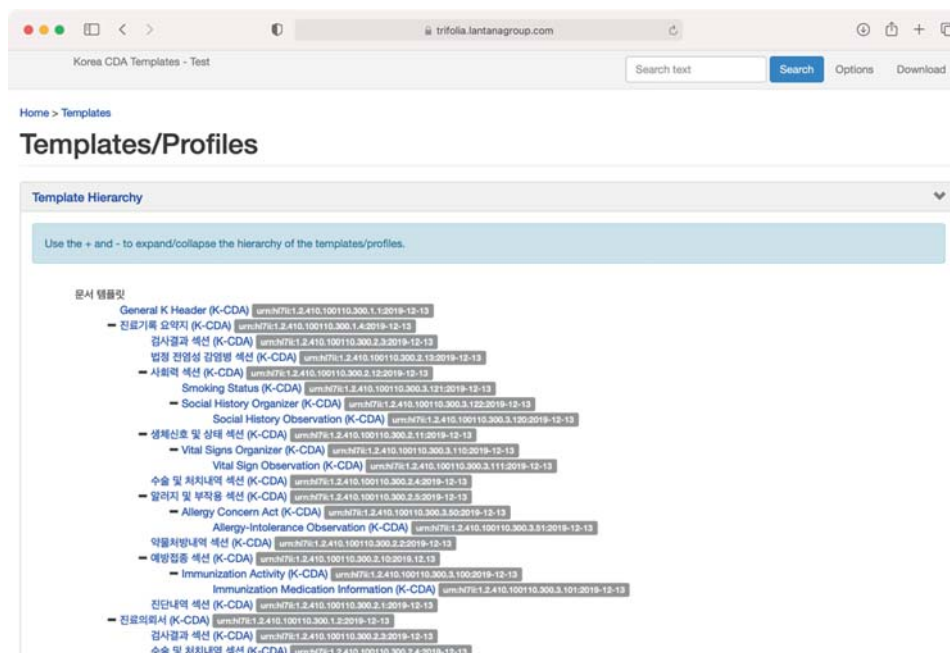
Fig. 3 Managing the CDA templates and automatic generation of Schematron through Trifolia Workbench. CDA, clinical document architecture.
