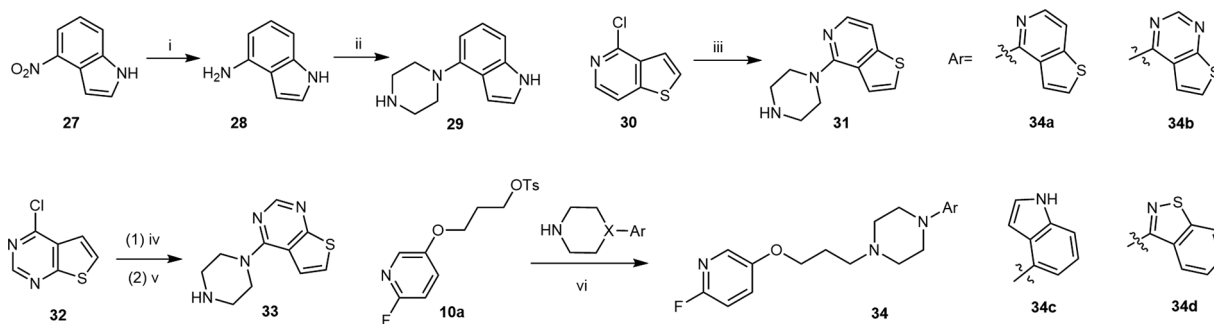
Scheme 4 Reagents and conditions: (i) Pd/C (10 wt %), \text{HCO}_2\text{NH}_4 , EtOH; (ii) 2,2'-dichloro-diethylamine hydrochloride, \text{K}_2\text{CO}_3 , isopropanol, 120^\circ\text{C} ; (iii) piperazine, ethylene glycol, 140^\circ\text{C} , 12 hours; (iv) 1-boc-piperazine, DIPEA, THF, r.t. (v) 5N HCl (aq); (vi) \text{K}_2\text{CO}_3 , \text{CH}_3\text{CN} , reflux.
