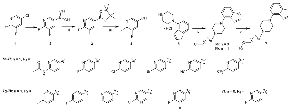
Scheme 1 The synthetic route for compounds 7a–7l . Reagents and conditions: (i) Pd 2 (dppf) 3 , PCy 3 , (BINP) 2 , CH 3 COONa, 1,4-dioxane, 85°C; (ii) pinacol, MgSO 4 , toluene, r.t.; (iii) H 2 O 2 , r.t.; (iv) 1-bromo-2-chloroethane or 1-bromo-3-chloropropane, K 2 CO 3 or 25% NaOH, r.t. or 60°C; (v) pyridine derivatives, K 2 CO 3 , CH 3 CN, reflux.
