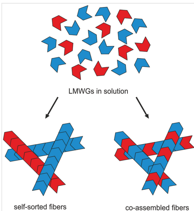
Figure 10 Self-assembly of multicomponent LMWGs, which can either self-sort into different fibers or co-assemble in the same fibers.
