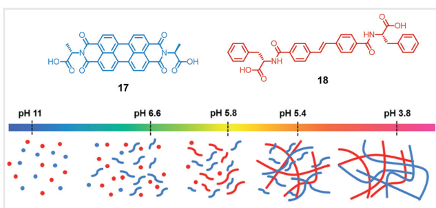
Figure 11 Molecular structures of the self-sorting building blocks 17 and 18 (top) Schematic representation of their stepwise self-assembly upon pH decrease (bottom). Adapted with permission from ref. 90. Copyright 2016 The Royal Society of Chemistry.
