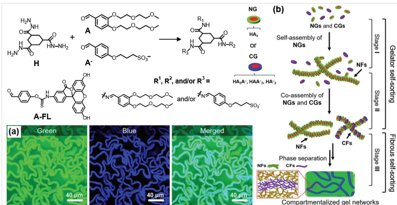
Figure 15 Molecular structures and the in situ synthesis of neutral and charged gelators. (a) CLSM images of macroscopic self-sorting. (b) Schematic illustration of the self-sorting process. A-FL and Hoechst 33342 were added for the visualization of green and blue fluorescence, respectively. Adapted and modified with permission from Ref. 103. Copyright 2019 American Chemical Society.
