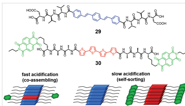
Figure 14 Molecular structures of gelators 29 and 30 . Their self-assembly is controlled by the acidification rates. Adapted with permission from Ref. 102. Copyright 2017 American Chemical Society.
