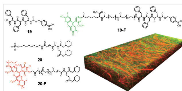
Figure 12 Molecular structures of the self-sorting building blocks 19 and 20 , and their corresponding fluorescent analogues 19-F and 20-F . Adapted with permission from Ref. 93. Copyright 2016 Nature Publishing Group.
