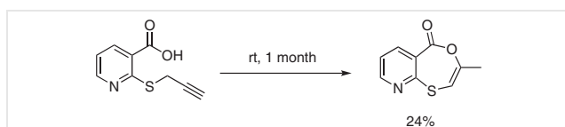
Scheme 1 Intramolecular conversion of 2-mercaptopyridine acid propargyl thioether
