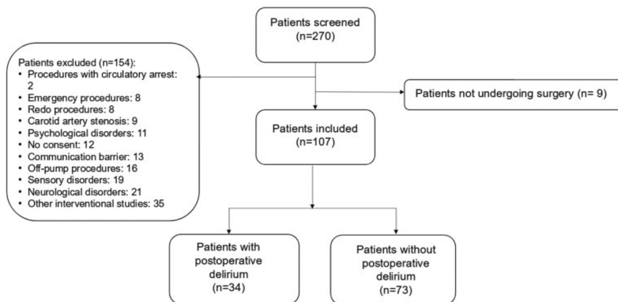
Fig. 1 Study design.
