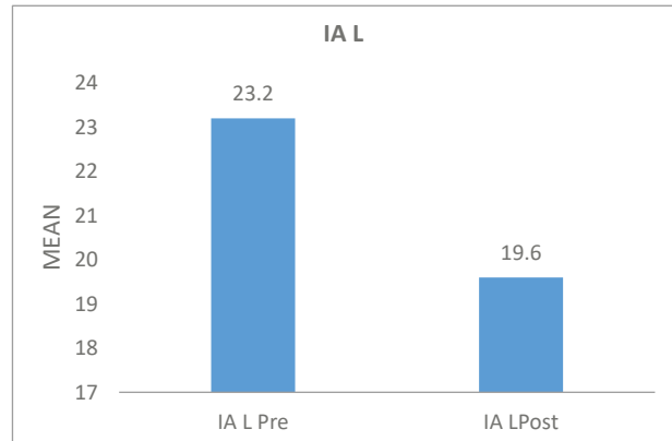
Graph 6 : Comparison of mean pretreatment and post treatment lower incisal angulations
