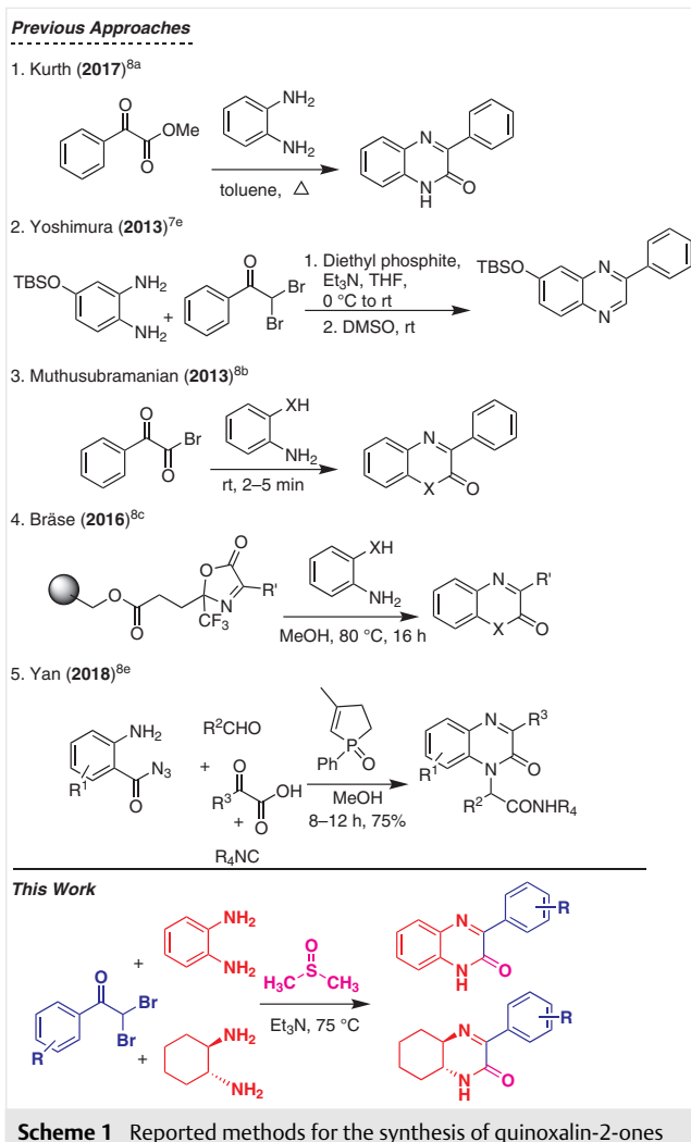
Scheme 1 Reported methods for the synthesis of quinoxalin-2-ones
