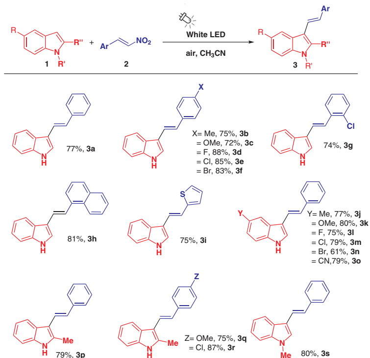
Scheme 2 Substrate scope. Reagents and conditions: indole 1 (1.5 mmol), (E)- \beta -nitrostyrene 2 (1 mmol), CH 3 CN (3 mL), irradiation using 7.0 W white LED in an open flask at r.t. Yield of the pure isolated products 3 .
