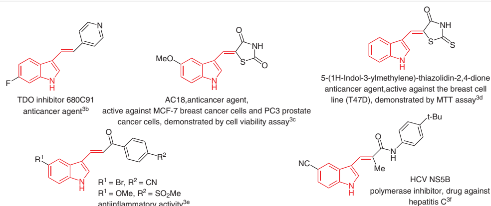
Figure 1 Some 3-alkenylindole-based therapeutic agents
