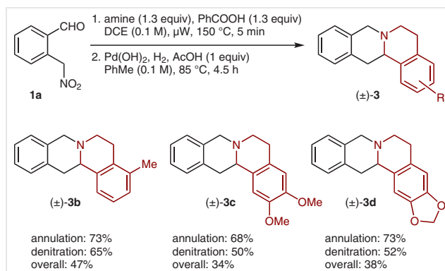
Scheme 3 Evaluation of substituted tetrahydroisoquinolines
