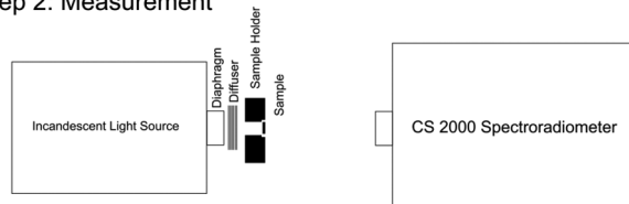
Fig. 2 Measurement of reflectance by a spectroradiometer.
