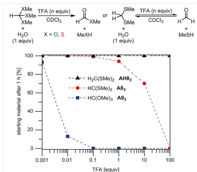
Figure 1 Effects of increasing amounts of TFA on the hydrolysis of orthoester (O,O,O)- A9 , trithioorthoester (S,S,S)- A8 , and dithioacetal AH8 . Reaction conditions: A9 or A8 or AH8 (37.5 \mu mol), increasing amounts of TFA [from 37.5 nmol (50 \mu M) to 3.75 mmol (5.0 M)], \text{CDCl}_3 ( V_{\text{total}} : 750 \mu L), r.t., 1 h; internal standard: toluene. For full spectra, see Figures S39–S56 in the SI.
