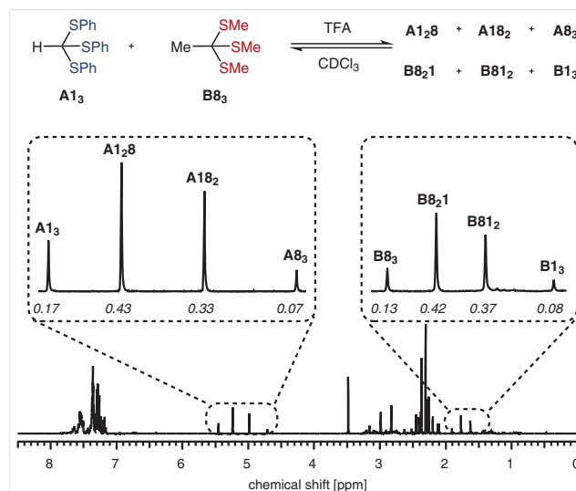
Figure 2 Trithioorthoester metathesis between A1 and B8 (top) and ^1\text{H} NMR spectrum measured after one hour (bottom). The two dashed boxes show the corresponding formate and acetoxy hydrogen atoms of trithioorthoesters formed from A1 and B8 . Reaction conditions: A1 (37.5 \mu mol), B8 (37.5 \mu mol), TFA (375 \mu mol), \text{CDCl}_3 ( V_{\text{total}} : 750 \mu L), r.t., 1 h. Product distributions are given by normalized integral values below the corresponding peaks for both sets. See also Table 2, entry 1 and the full spectra in Figure S59 in the SI.
