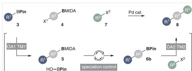
Scheme 10 Design plan for a sequential chemoselective Suzuki-Miyaura cross-coupling
