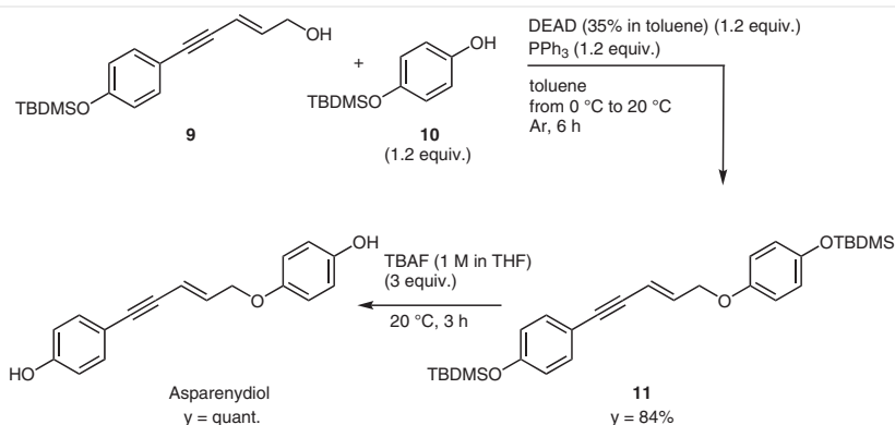
Scheme 5 Mitsunobu etherification to synthesize intermediate 11 and deprotection to form Asparenediol ( 15 )
