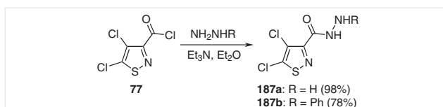
Scheme 65 Preparative synthesis of hydrazides of 4,5-dichloroisothiazole-3-carboxylic acid
