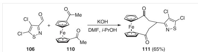
Scheme 44 Design of ferrocenyl containing isothiazoles
