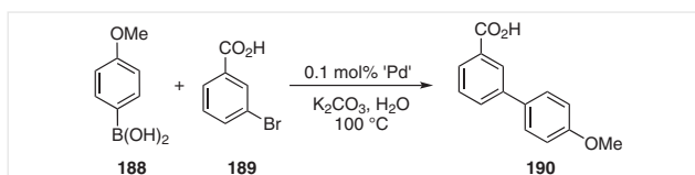
Scheme 66 Model reaction - synthesis of 4'-methoxy[1,1'-biphenyl]-3-carboxylic acid
