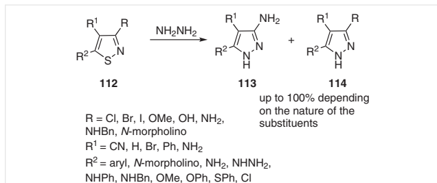
Scheme 45 Conversion of isothiazoles into aminopyrazoles
