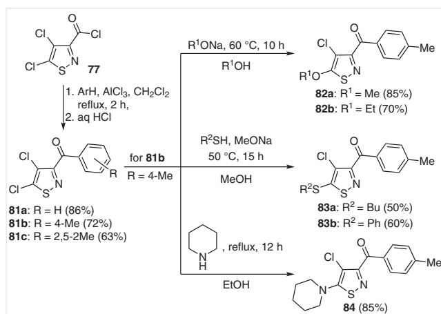
Scheme 35 Preparation of 3-ketoderivatives of 4,5-dichloroisothiazole
