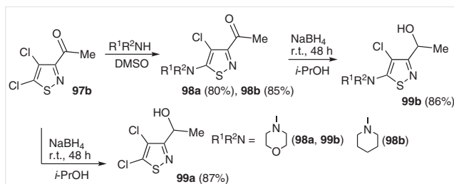
Scheme 40 Some transformations of 3-acetyl-4,5-dichloroisoithiazole
