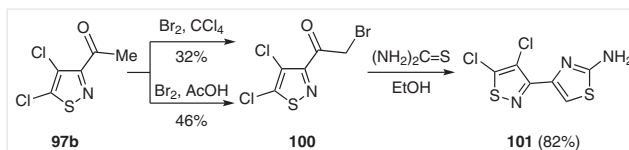
Scheme 41 Modification of the acyl substituent in (4,5-dichloroisoithiazol-3-yl) methyl ketone
