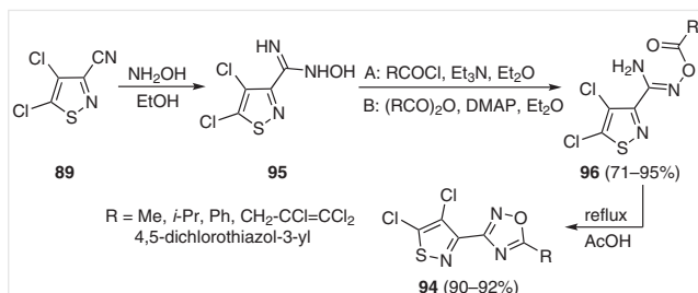
Scheme 38 Transformation of the nitrile group in 3-cyano-4,5-dichloroisoithiazole to 1,2,4-oxadiazole ring
