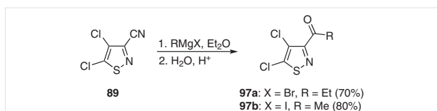
Scheme 39 Preparation of 3-alkylketo-4,5-dichloroisoithiazoles
