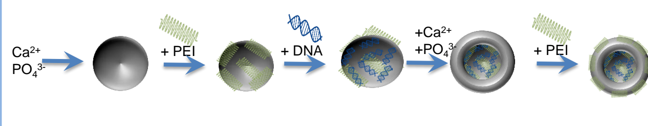
Fig. 3: CaP nanoparticles were precipitated by dropwise addition of \text{Ca}^{2+} and \text{PO}_4^{3-} solutions. A defined volume was then combined with pDNA solution, stabilizing the particles. For cell studies with dispersions, triple-shell particles were precipitated with PEI and DNA, additional protection of the DNA was accomplished by a layer of CaP and polyethylenimine (PEI) on the surface.
