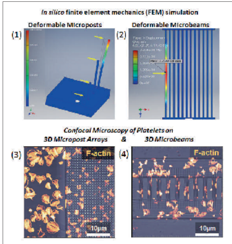
Fig. 2 In silico finite element mechanics (FEM) simulation. Deformable Microbeams (OC 6.3)
