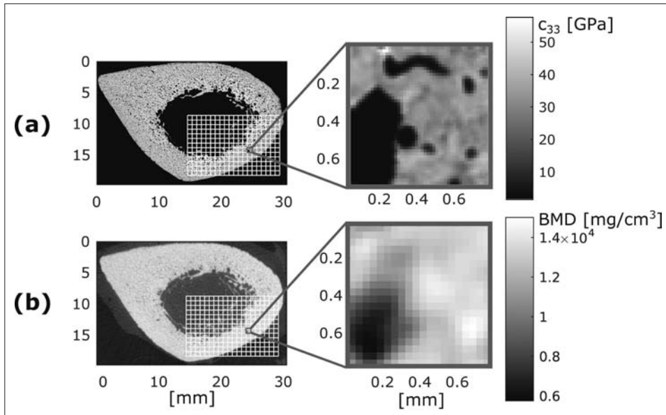
Fig. 1: SAM (a) and registered \mu CT (b) images with a detail of the same ROI (right). The isotropic 2D grid [grid size: 740 \mu m] can be appreciated. As the spatial resolution of the SAM images was better than that of the \mu CT images, the segmentation of pores (Haversian canals and basic remodeling units) from the tissue matrix was performed on the SAM images using a global threshold [ Z = 5 Mrayl]. While the periosteal surface was segmented automatically, the endosteal surface was defined manually. Mean BMD was obtained for each \mu CT ROI, while mean Ct.Po and c33 were extracted for the corresponding SAM ROI.
