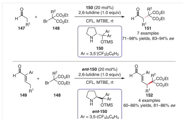
Scheme 64 Enantioselective alkylation of aldehydes and enals
