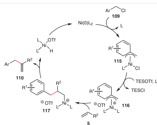
Scheme 17 Jamison's mechanism for the Ni-catalyzed Heck reaction of benzylic chlorides
