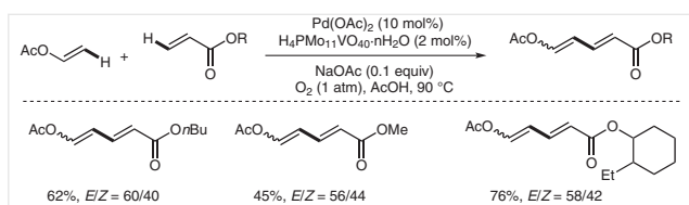
Scheme 2 Oxidative cross-coupling of acrylates with vinyl carboxylates
