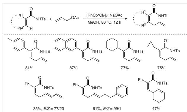
Scheme 10 Rhodium-catalyzed allylation of acrylamides
