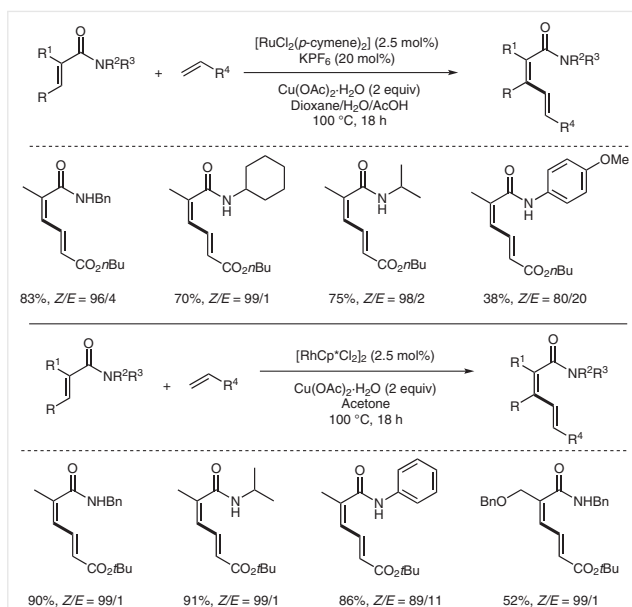
Scheme 9 Ruthenium-catalyzed weak directing-group-enabled alkynyl \text{sp}^2 C–H activation
