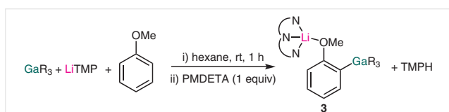
Scheme 3 Synthesis of [(PMDETA)Li( o -C 6 H 4 OMe)Ga(CH 2 SiMe 3 ) 3 ] ( 3 )
