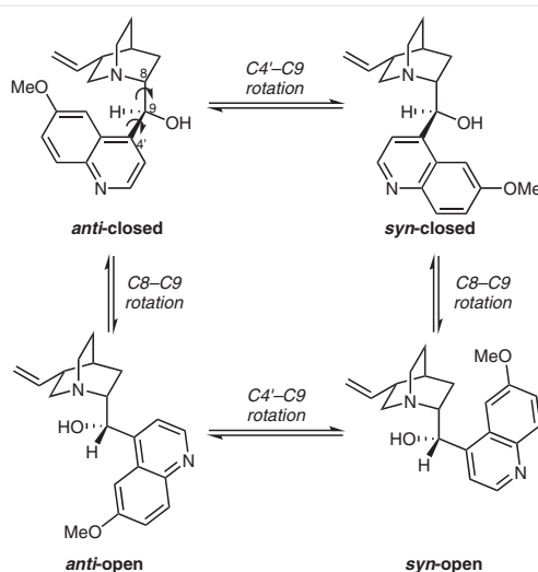
Scheme 5 Four accessible conformations of quinidine. There have been up to 7 major conformations reported in the literature
