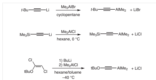
Scheme 1 Preparation of dimethylalkynylaluminum reagents by transmetalation
