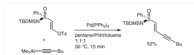
Scheme 28 Stereospecific synthesis of enynylsulfoximines
