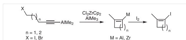
Scheme 30 Intramolecular reaction of bis-metalated reagents
