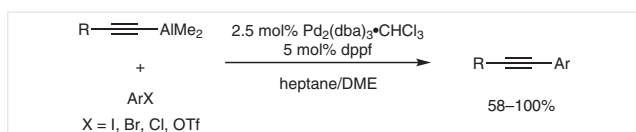
Scheme 26 Palladium-catalyzed cross-coupling reactions
