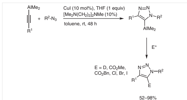
Scheme 31 Copper-catalyzed 3+2 cycloaddition of azides with dimethylalkynylaluminum reagents and subsequent transformations
