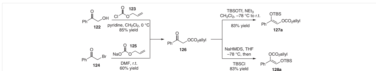
Scheme 43 An efficient regiodivergent synthesis of Pd-DAAA substrates
