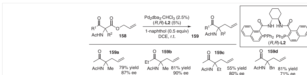
Scheme 55 Pd-DAAA of \alpha -acetamido- \beta -keto esters
