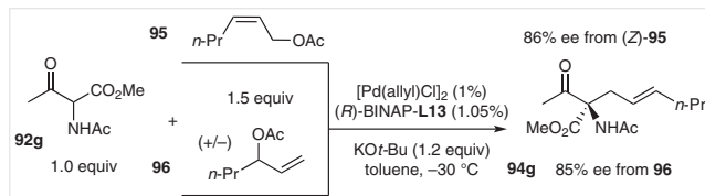
Scheme 31 Independence of electrophile regio- and stereochemistry on reaction outcome
