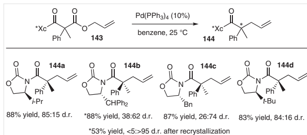
Scheme 49 Auxiliary approach for the Pd-DAA of acyclic allyl \beta -oxo esters
