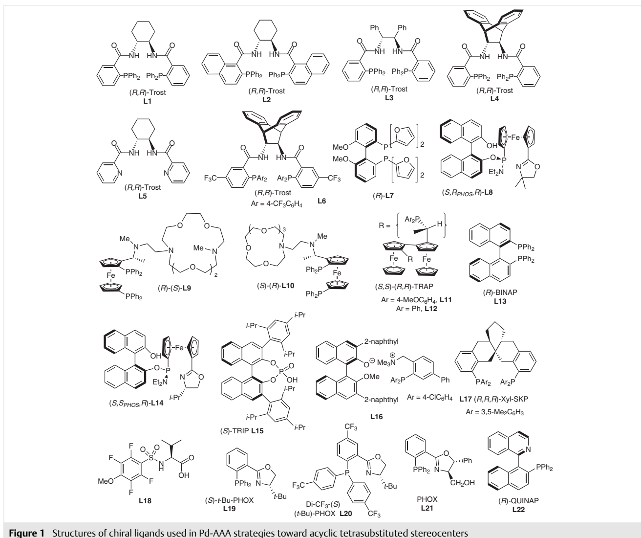
Figure 1 Structures of chiral ligands used in Pd-AAA strategies toward acyclic tetrasubstituted stereocenters
