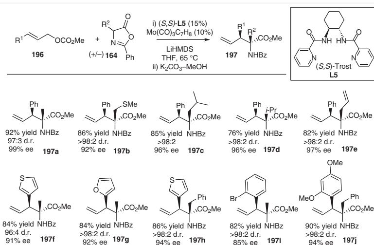
Scheme 67 One-pot Mo-catalyzed regio-, diastereo-, and enantioselective allylic alkylation of azlactones followed by hydrolysis
