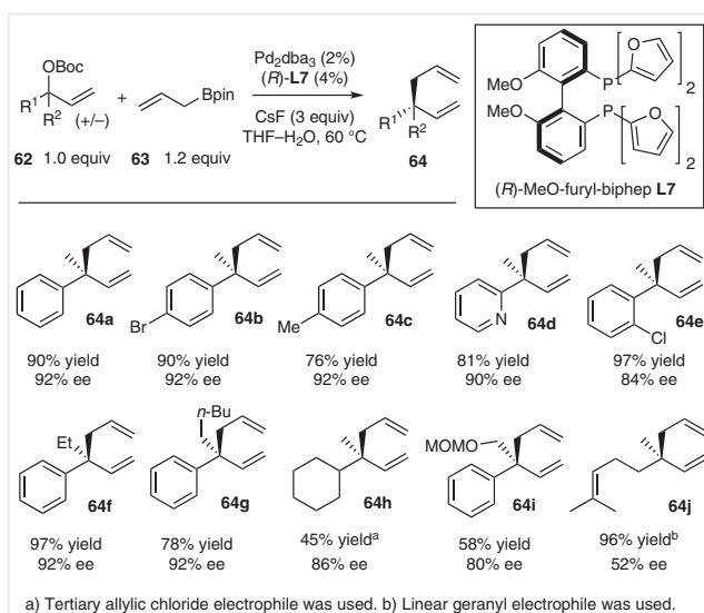
Scheme 23 Catalytic enantioselective branch selective allyl-allyl cross coupling
