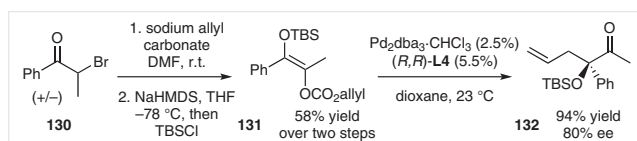
Scheme 46 Synthesis and reaction of ketone-derived \alpha -alkoxy enol carbonate
