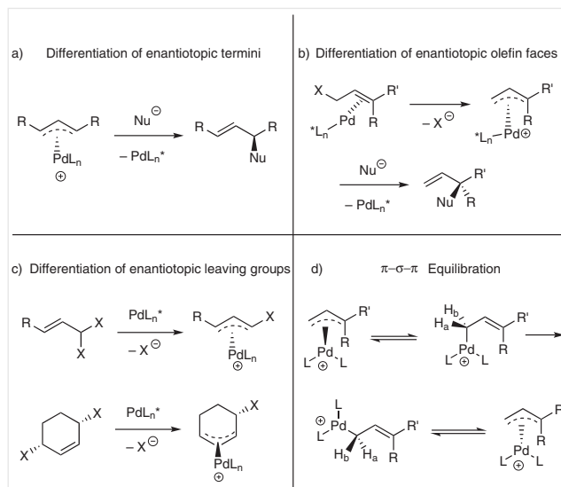
Scheme 3 Modes of asymmetric induction on electrophile
