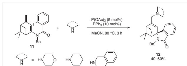
Scheme 9 Racemic intramolecular arylation/amination
