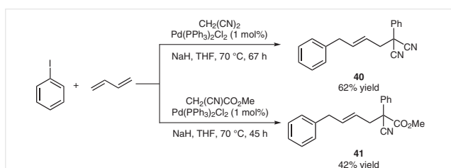
Scheme 27 Arylation with iodobenzene
