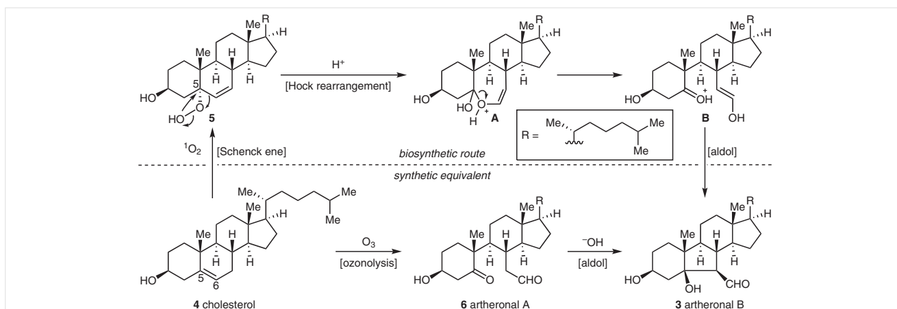
Scheme 1 Biosynthetic route (top) and synthetic equivalent (bottom) to the metabolites atheronal A ( 6 ) and atheronal B ( 3 )
