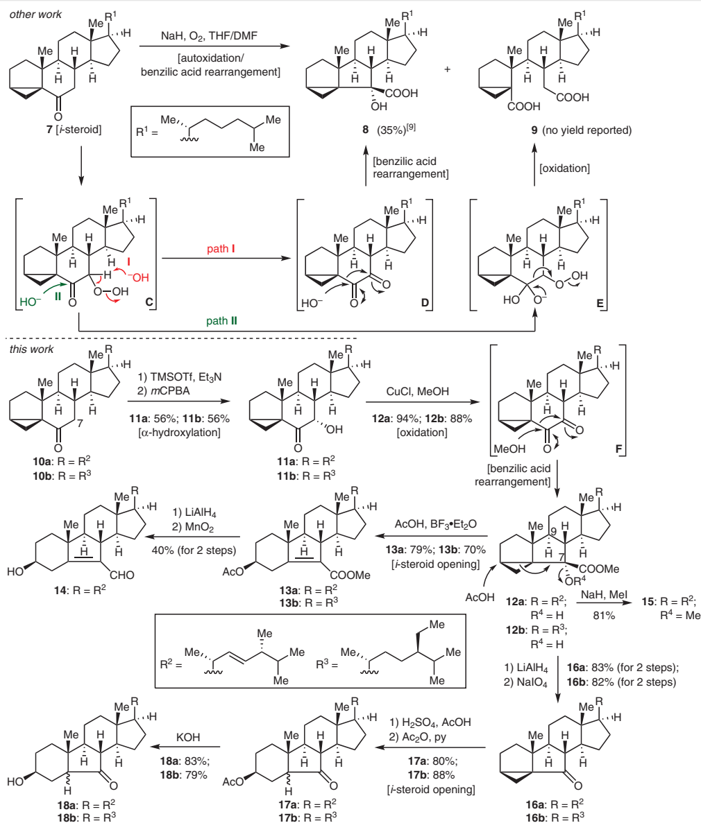
Scheme 2 Liang's autoxidation–rearrangement procedure for the benzilic acid rearrangement of cholesterol-derived 7 (top) and this work's approach (bottom)
