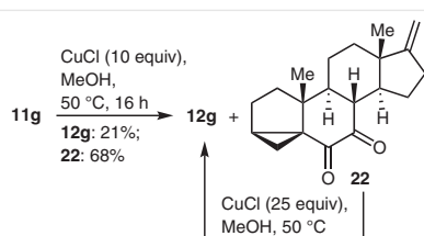
Scheme 4 Synthesis of dione intermediate 22 and its conversion into 12g
