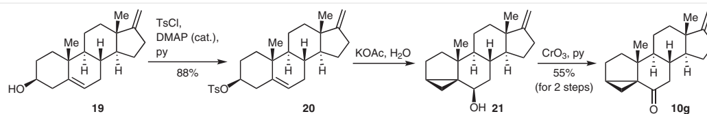
Scheme 3 Synthesis of substrate 10g
