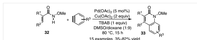
Scheme 16 Quinolinones from annulation between acrylamides and arynes
