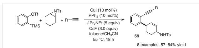
Scheme 34 Three-component coupling of benzyne, terminal alkyne, and vinylaziridine in the presence of CuI
