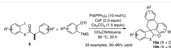
Scheme 6 Pd-catalyzed spirocyclization
