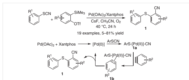
Scheme 2 2-(Arythio)benzotriles from insertion of arynes into aryl thiocyanates catalyzed by Pd(OAc) 2
