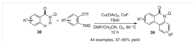
Scheme 19 Phenanthridinone by Cu-catalyzed annulations of aryne, and benzamides; Q = 8-quinoliny
