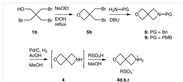
Scheme 7 Synthesis of 2-oxa-6-azaspiro[3.3]heptane sulfonate salts
