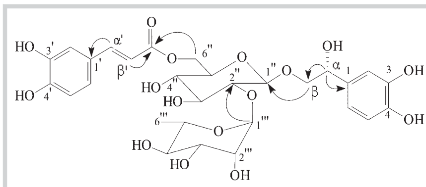
Fig. 1 Key HMBC correlations (H → C) of 1.
