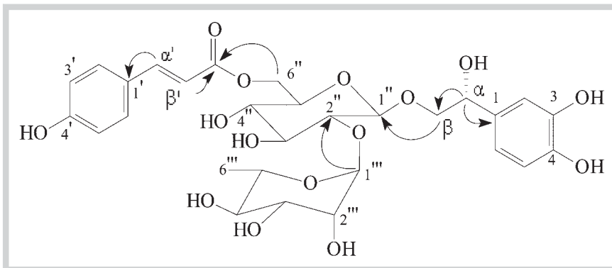
Fig. 4 Key HMBC correlations (H → C) of 4 .
