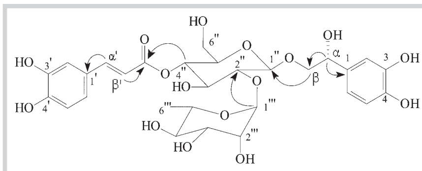
Fig. 2 Key HMBC correlations (H → C) of 2.
