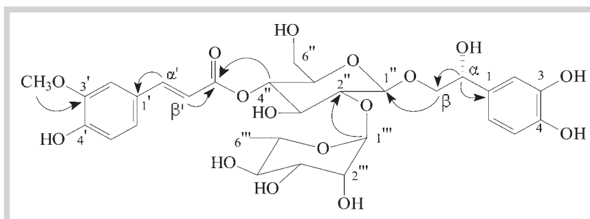
Fig. 3 Key HMBC correlations (H → C) of 3.
