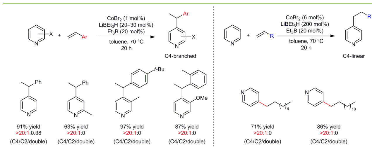
Scheme 2 Representative examples
