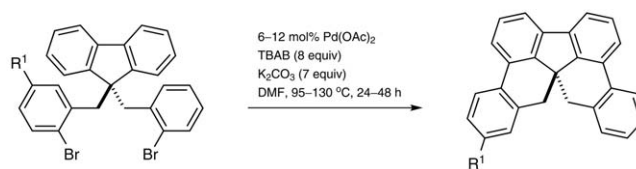
Scheme 17 Palladium-catalyzed double C–H activation–cyclization to a polycyclic aromatic molecule
