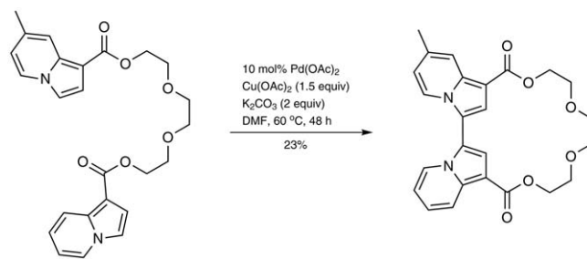
Scheme 20 Macrocycle synthesis by palladium-catalyzed double C–H activation
