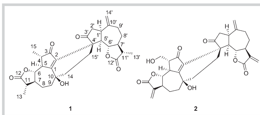
Fig. 1 Structures of compounds 1–2.
