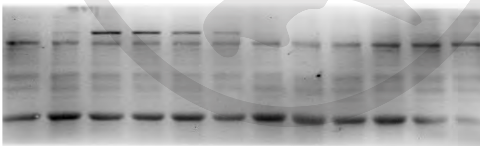
Btk Y223
