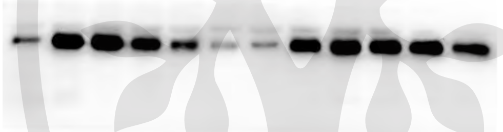
LAT Y220
