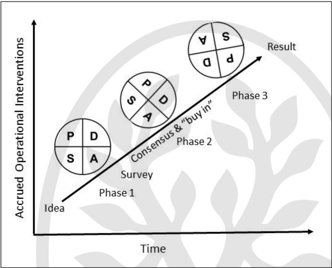
Figure 1) PDSA Ramp
