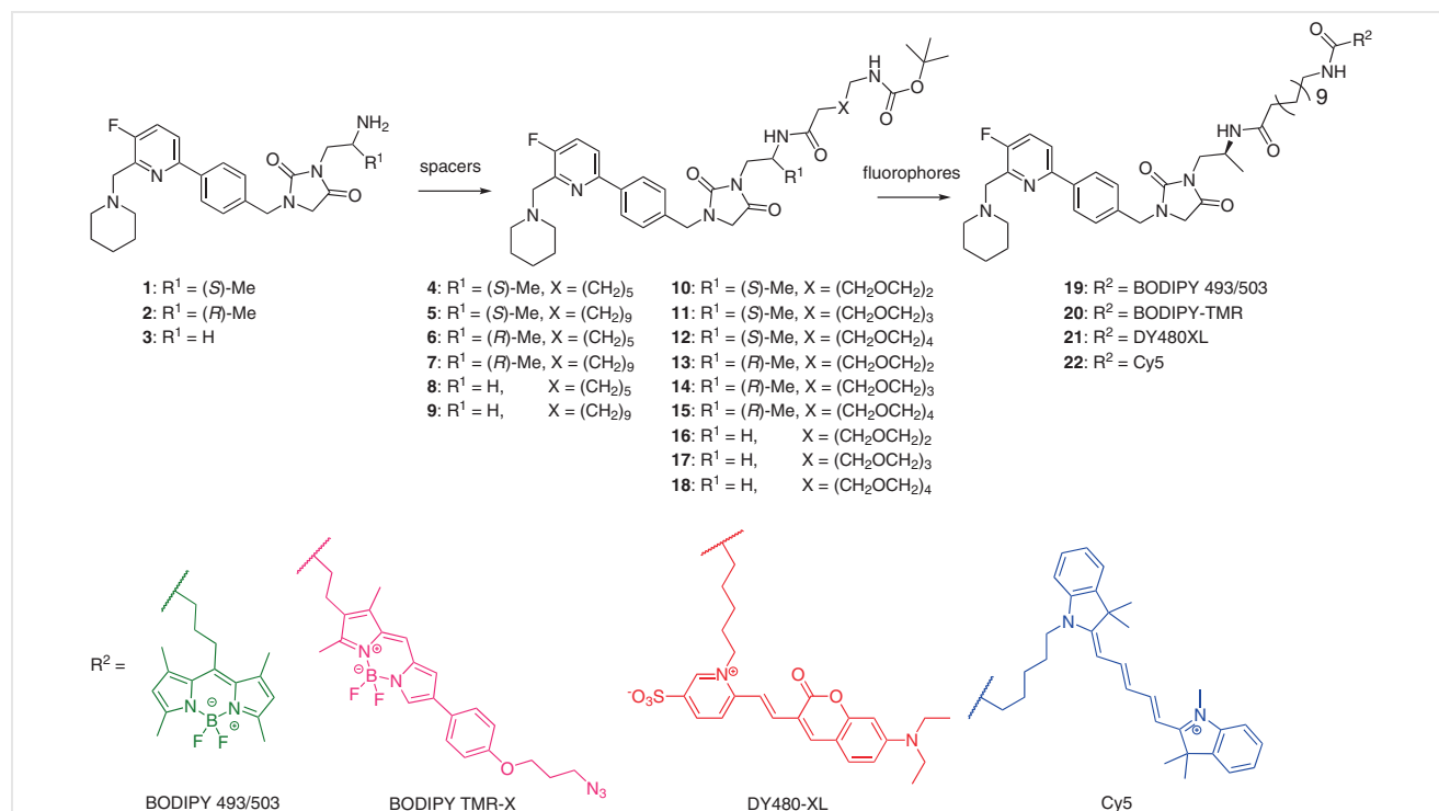
Scheme 1 The synthesis plan for the LEI-102-derived fluorescent probes. The scaffold contains an amine conjugation site that is either the ( S )- or ( R )-2-aminopropyl enantiomer or achiral 2-aminoethyl moiety. To all three scaffolds a selection of five spacers was conjugated: C 8 , C 12 , PEG 2 , PEG 3 , or PEG 4 . Compound 5 exhibited the highest CB 2 R affinity and was conjugated to the four fluorophores. The Cy5 conjugate 22 showed the best biochemical properties.
