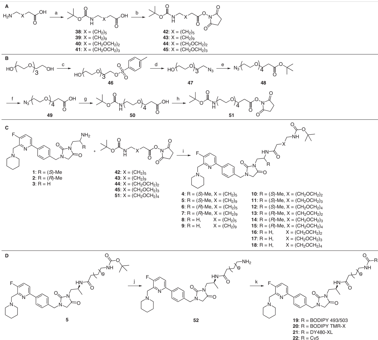
Scheme 3 The synthesis of the 15 intermediates followed by the synthesis of the fluorescent probes. Reagents and conditions: (a) Alkyl : Et 3 N (2 equiv), Boc 2 O (1.1 equiv), acetone/H 2 O (1:1, v/v, 0.5 M), r.t., 16 h, 95–99%; PEG : K 2 CO 3 (3 equiv), Boc 2 O (1.3 equiv), H 2 O/THF (1:1, v/v, 0.1 M), r.t., 16 h, 40–81%; (b) Alkyl : EDC·HCl (0.8–0.9 equiv), NHS (1.7–2.8 equiv), DCM (0.3 M), r.t., 16–72 h, 36–40%; PEG : EDC·HCl (3 equiv), NHS (1.5 equiv), Et 3 N (3 equiv), DCM (0.2 M), r.t., 16 h, 46–58%; (c) p -TsCl (1 equiv), NaOH (2 M, 1.6 equiv), THF (0.6 M), 0 °C, 4 h, 90%; (d) NaN 3 (1.5 equiv), ACN (0.4 M), 80 °C, 8 h, 94%; (e) tert -butyl acrylate (1 equiv), TBAF (0.4 equiv), NaOH (25 wt% in H 2 O, 2.6 equiv), DCM, r.t., 8 h, 75%; (f) TFA (50 equiv), DCM, r.t., 4 h, 65%; (g) step 1: 10% Pd/C (0.1 equiv), H 2 gas, EtOH (0.3 M), r.t., 16 h; step 2: K 2 CO 3 (3 equiv), Boc 2 O (1.3 equiv), H 2 O/THF (1:1, v/v, 0.1 M), r.t., 16 h, 55% (two steps); (h) EDC·HCl (1.2 equiv), NHS (1.1 equiv), DCM (0.2 M), r.t., 16 h, 84%; (i) Et 3 N (6 equiv), DCM (0.3 M), r.t., 1–3 h, 13–65%; (j) TFA (110 eq), DCM, r.t., 2 h, quant.; (k) 19–21 : Et 3 N (1 equiv), fluorophore-NHS ester (1 equiv), CH 2 Cl 2 (0.3 M), r.t., 1–3 h, 64–100%; 22 : HOBT (1.2 equiv), DIPEA (2.5 equiv), EDC·HCl (1.3 equiv), cyanine-5-carboxylic acid (1.1 equiv), DMF (0.007 M), r.t., 16 h, quant.
